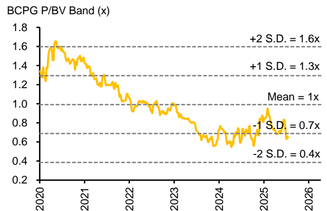
Fig 4: BCPG Forward PBV Band
