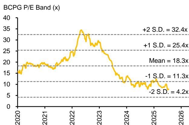
Fig 3: BCPG Forward PE Band
