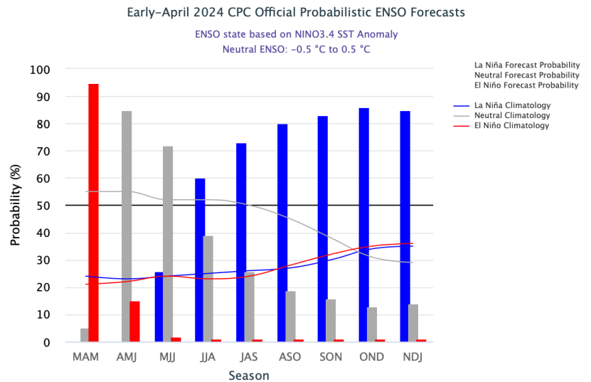
Figure 2: 60% probability of La Nina conditions from June 2024
