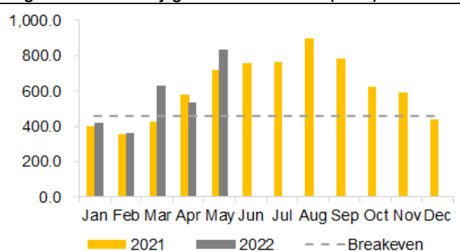
Figure 4: Electricity generation at XPCL (GWh)
