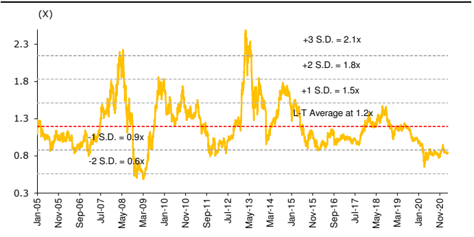
Figure 3: P/BV band
