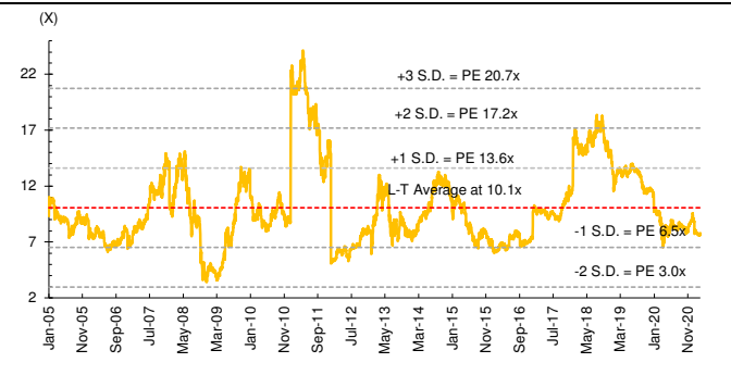
Figure 2: PER band
